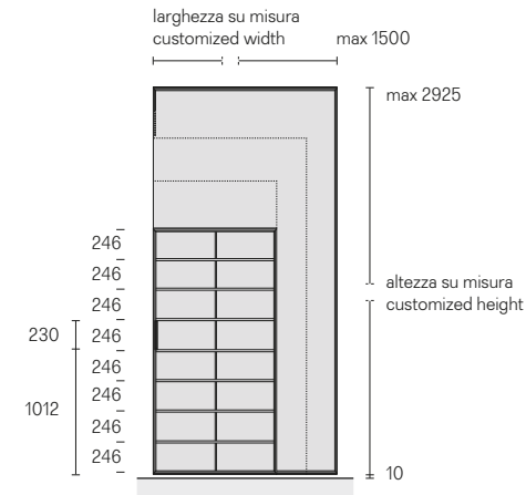
Dimensioni pannelli scorrevoli Sliding panel dimensions
